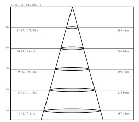
Height: 100mm | Plane beam angle: 90.0 deg | Spot Diameter: 115.14mm
